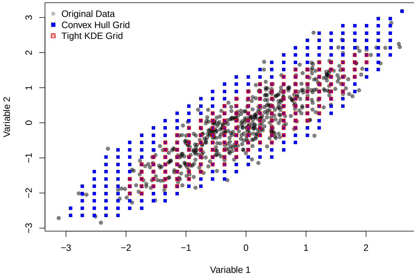
KDE Density (Red) vs. Convex Hull (Blue)
