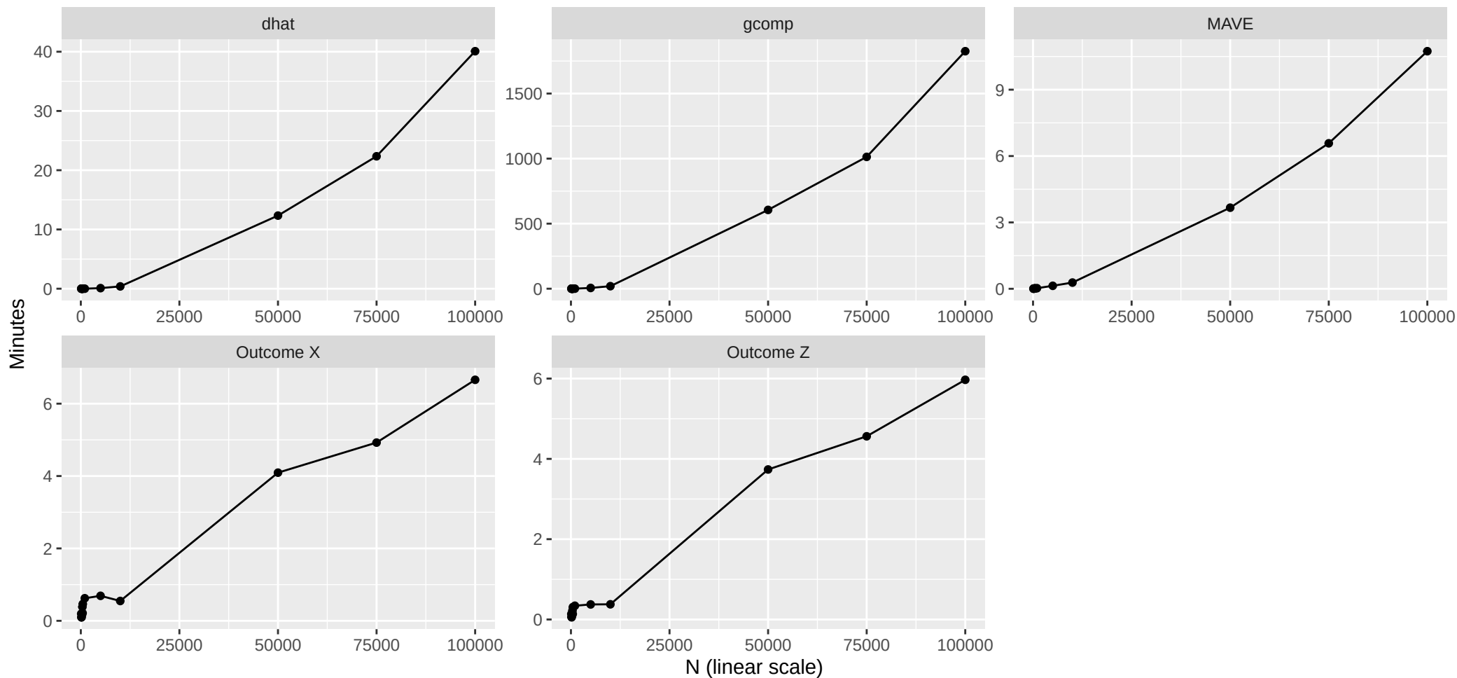
Runtimes (min) for different components of causal SDR
