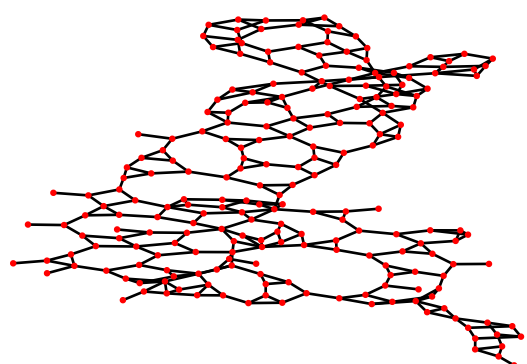
Fungal growth networks
