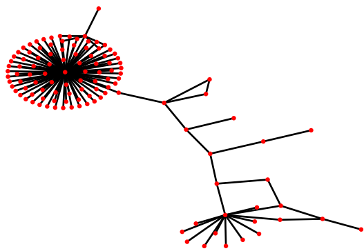
C. elegans interactomes (2009)
