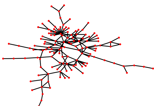
Binary interactomes (various species; 2012)
