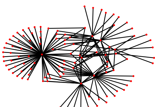
Barrett & Helenurm plant-pollinator web
