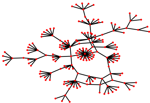
Norwegian Boards of Directors (2002-2011, bipartite)
