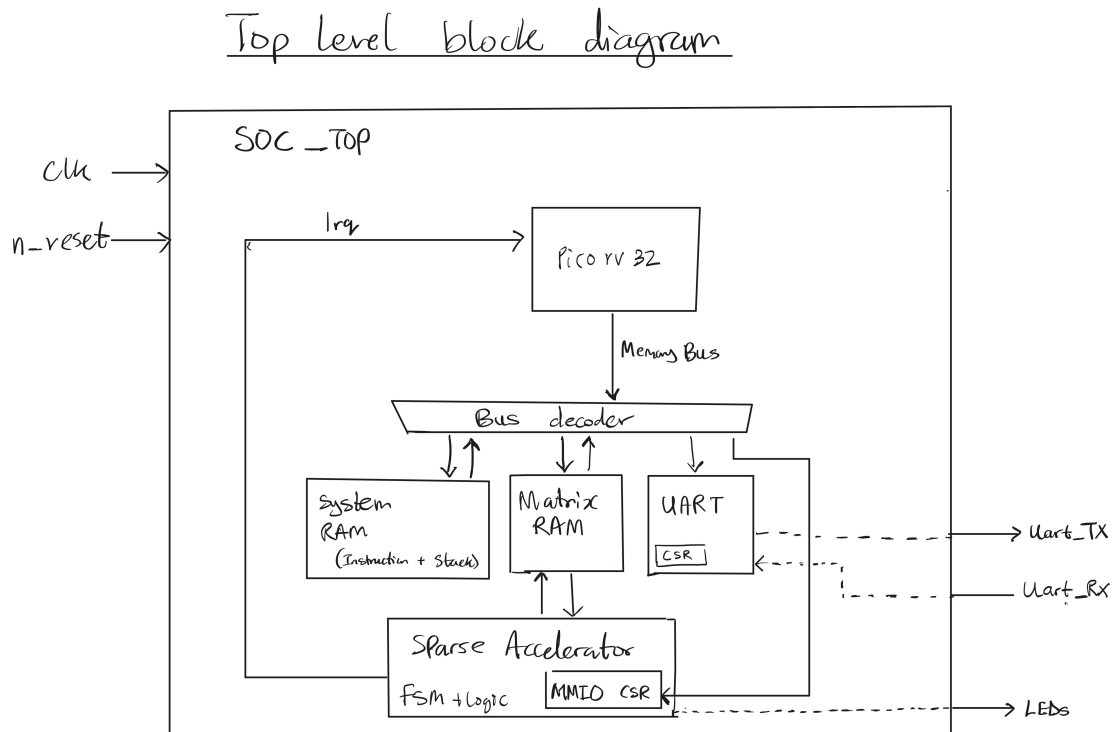
FIGURE 3.1: Top-level RISC-V SoC block diagram.
