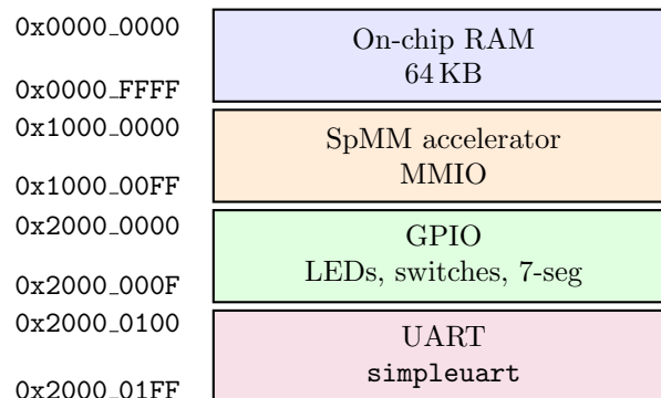
FIGURE 3.3: System memory map as a vertical address strip.
