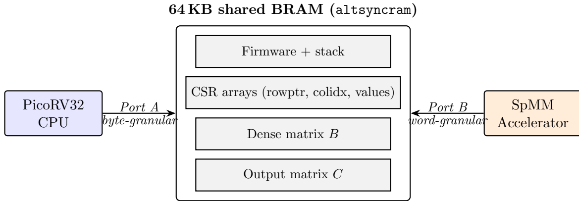
FIGURE 3.2: Dual-port BRAM organisation.
