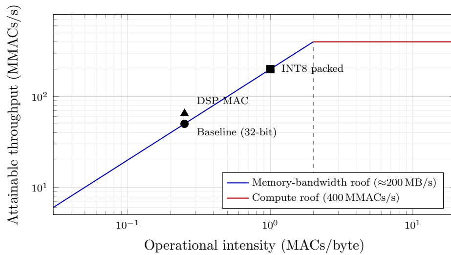
FIGURE 2.3: Roofline interpretation of the three accelerator stages on the Cyclone V platform. INT8 packing raises the operational intensity by a factor of four, shifting the design rightward and upward along the bandwidth roof towards the compute-bound region.
