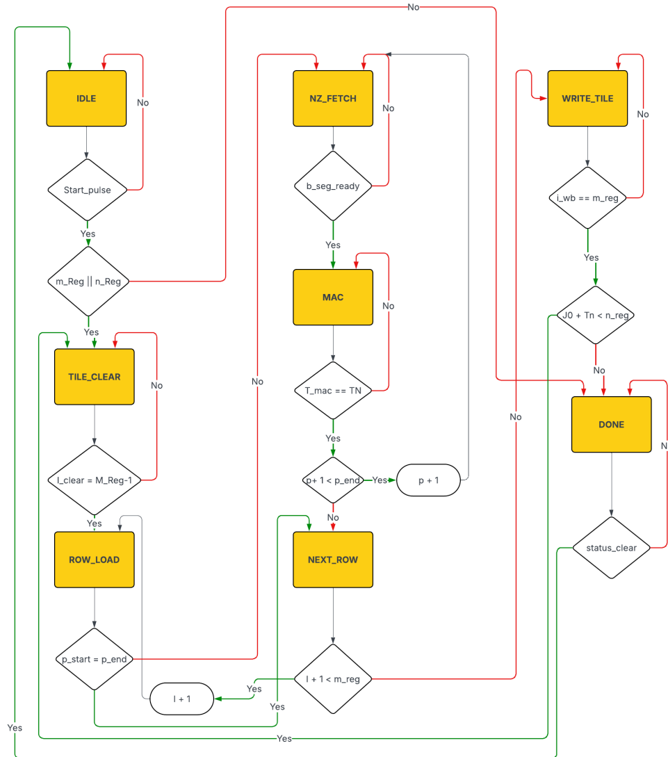
FIGURE 4.3: Simplified accelerator finite state machine. Each major phase corresponds to one row in Table 4.1. Sub-phase transitions within ROW_LOAD and NZ_FETCH absorb the one-cycle registered RAM output latency.
