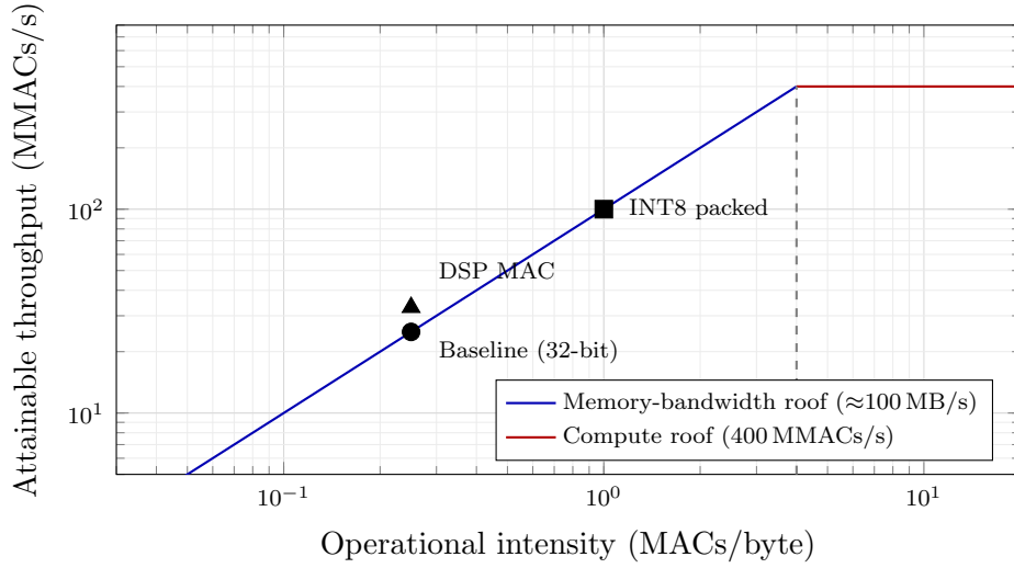
FIGURE 2.4: Roofline interpretation of the three accelerator stages on the Cyclone V platform. The baseline and DSP-enhanced designs sit on the memory-bandwidth roof: arithmetic throughput is capped by operand fetch, so widening the MAC array yields only a small gain. INT8 packing raises the operational intensity by a factor of four (four operands per 32-bit word), shifting the design rightward and upward along the bandwidth roof towards the compute-bound region.
