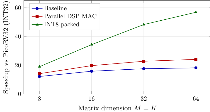
FIGURE 6.1: Speedup versus matrix size for tests T1–T4 (fixed N = 8 , 75% uniform sparsity). Larger matrices amortise fixed setup overhead, with the INT8 stage giving the largest absolute gain.
