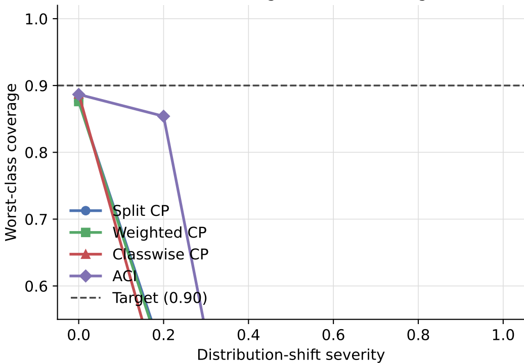
Worst-class coverage under increasing shift
