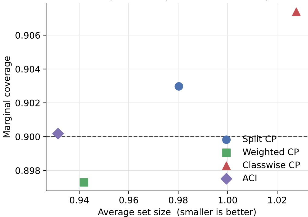
Coverage-efficiency trade-off at severity 1
