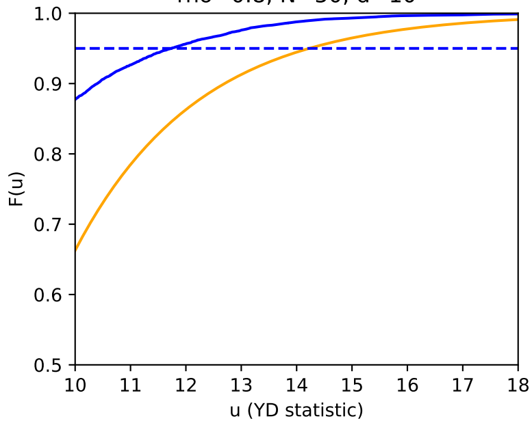
\rho=0.8, N=50, d=10
