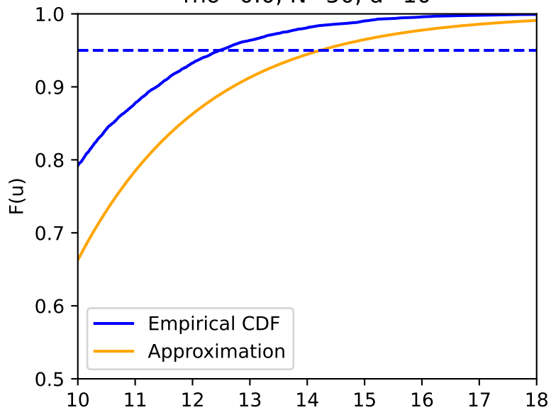
\rho=0.0, N=50, d=10
