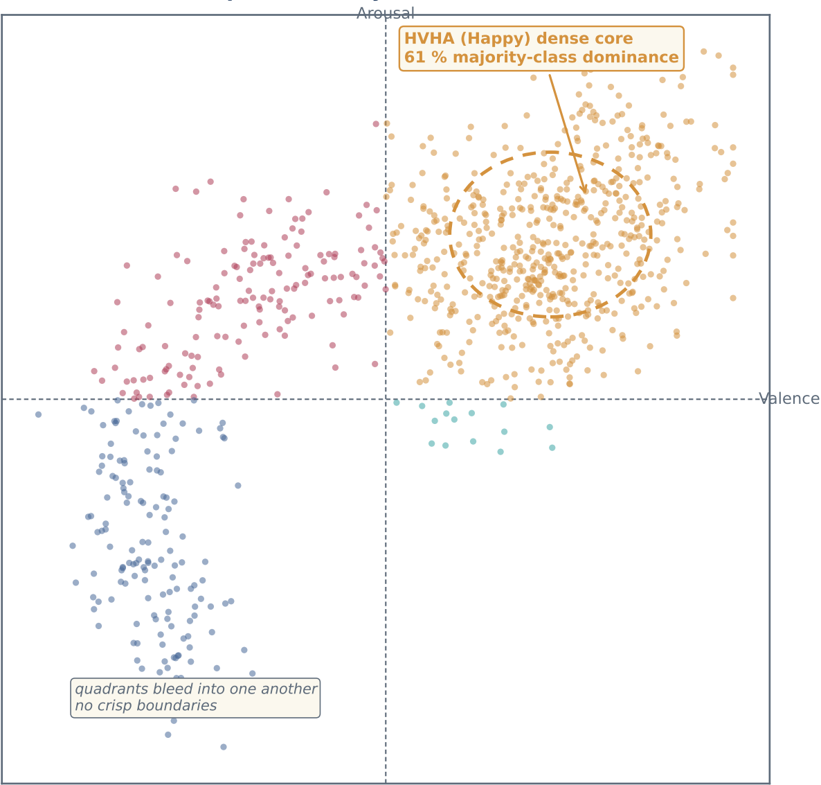
(b) The Empirical Reality — Continuous Manifold
