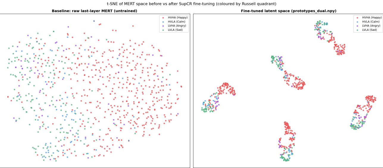
Fig. 1 — t-SNE of the song space. Left: raw untrained MERT is one mixed blob (no emotion separation). Right: after training, clear structure appears but it is a continuous, Happy-dominated manifold, not four clean clusters.
