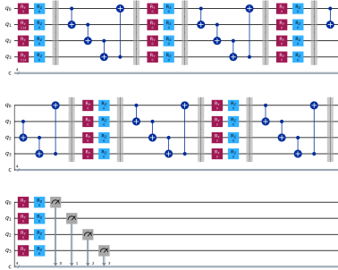
(a) Sirkuit (GT)
