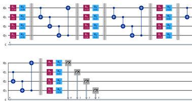
(a) Sirkuit (GT)
