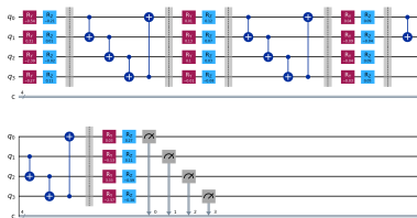
(b) Sirkuit (No-GT)
