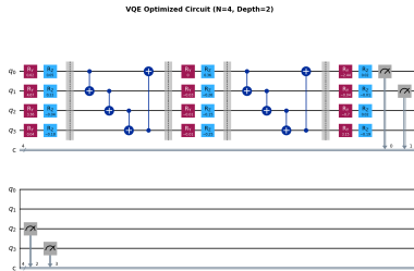
(a) Sirkuit (GT)
