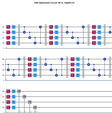
(b) Sirkuit (No-GT)
