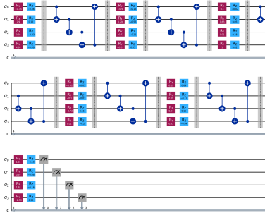
(a) Sirkuit (GT)
