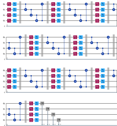
(b) Sirkuit (No-GT)
