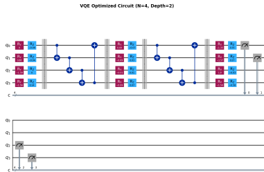
(b) Sirkuit (No-GT)
