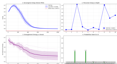
Analisis VQE Warm-Start - Jendela 2023-11-03 (N=6, K=3)
