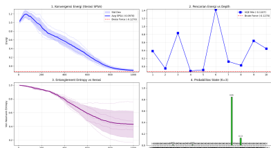
Analisis VQE Warm-Start - Jendela 2022-06-23 (N=6, K=3)
