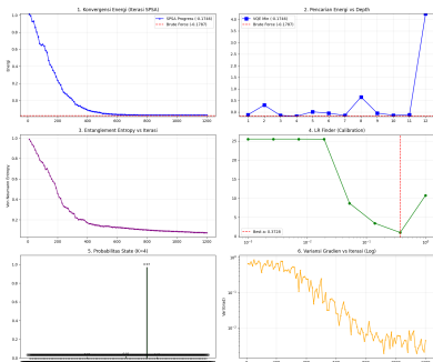
Analisis VQE Warm-Start - Jendela 2022-06-23 (N=8, K=4)
