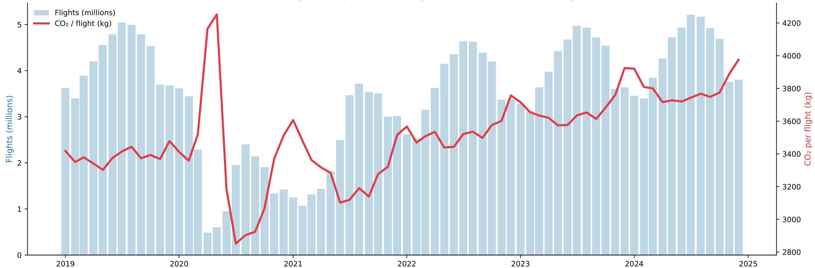
CO 2 efficiency per flight vs total flight volume — ECAC monthly
