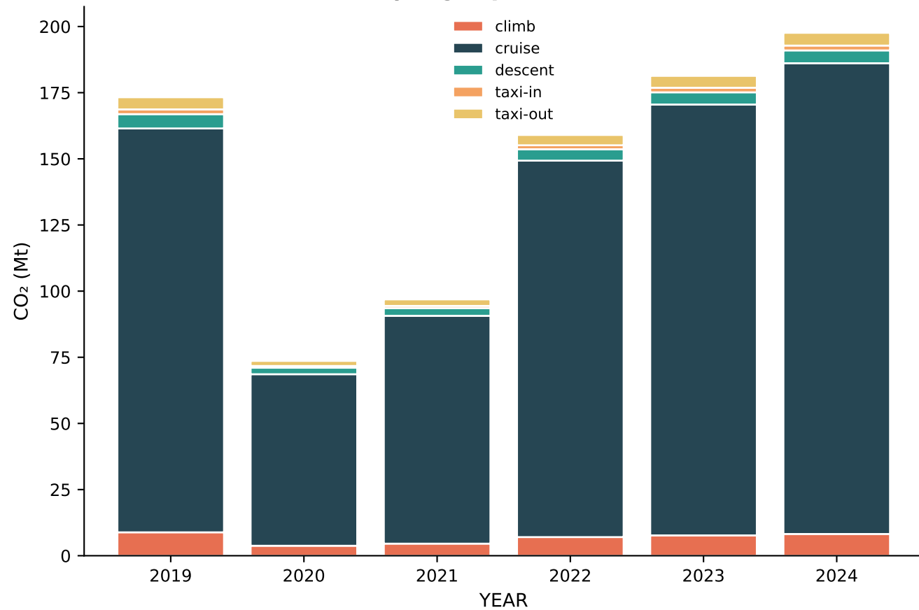
CO 2 by flight phase absolute
