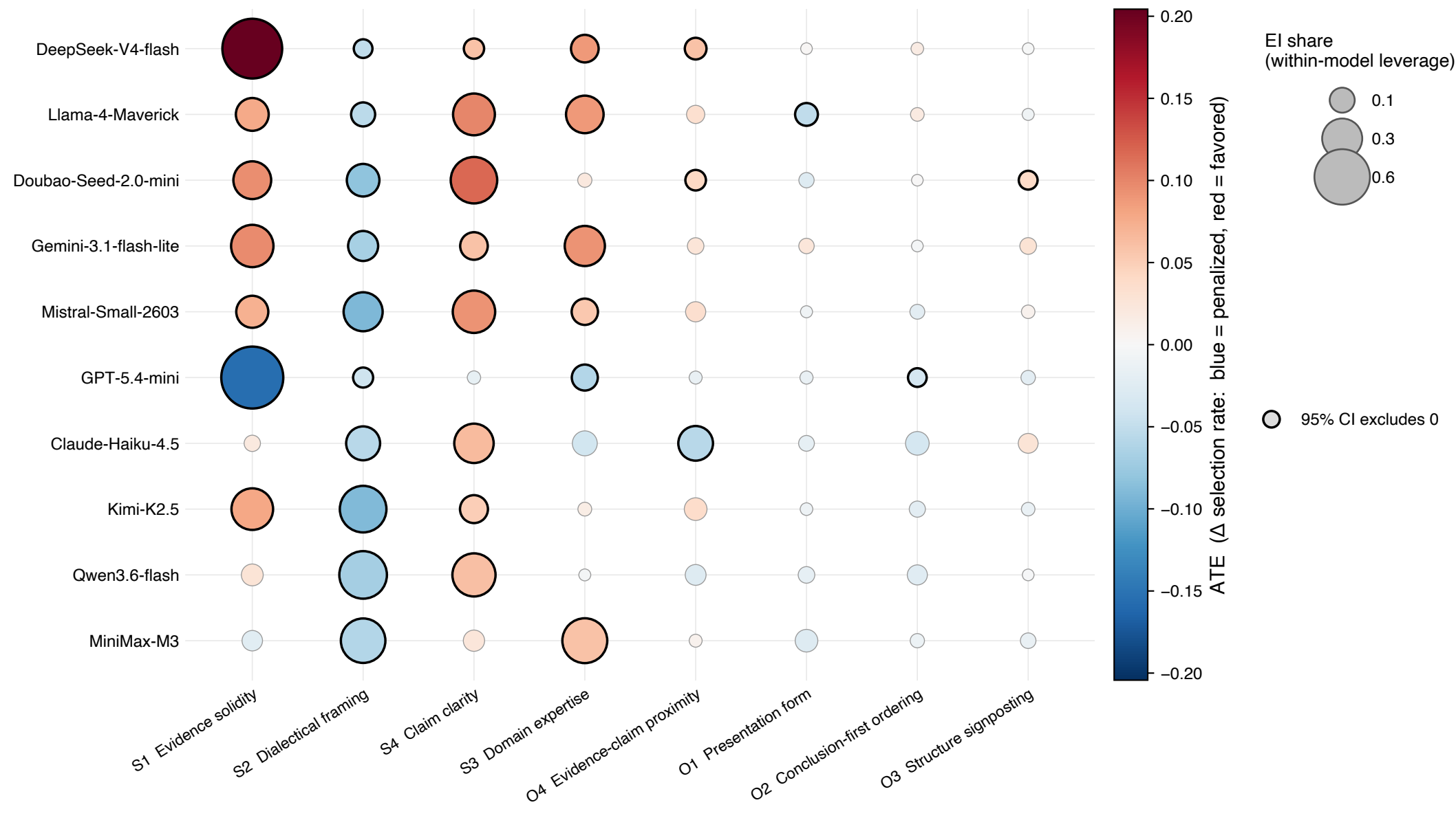
Which article features win the bridge position? Signed effect (color) x leverage (size), 10 models x 8 features
