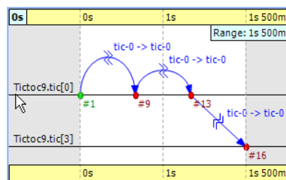
Figure 8.17. Filtering for node '0' and '3'
