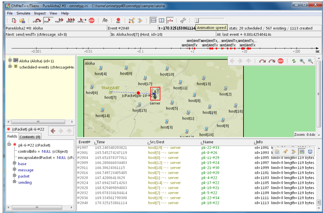
Figure 7.1. The main window of Tkenv
