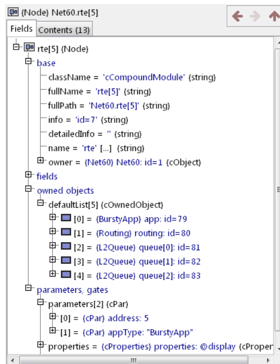
Figure 7.12. The object inspector
