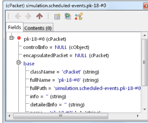
Figure 7.6. A floating inspector window
