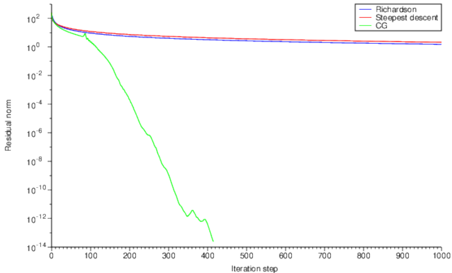
CG method applied to the discretization of the Laplace operator
