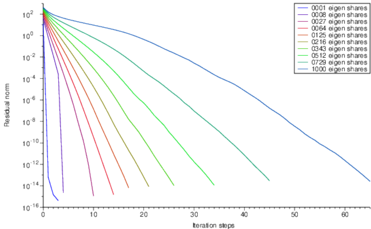
CG method with different right hand sides, highest eigenvalues
