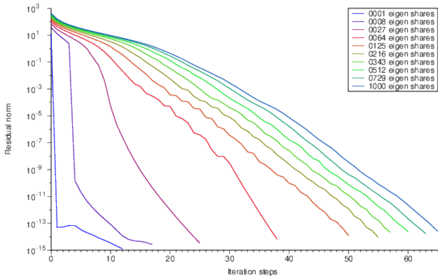
CG method with different right hand sides, lowest eigenvales
