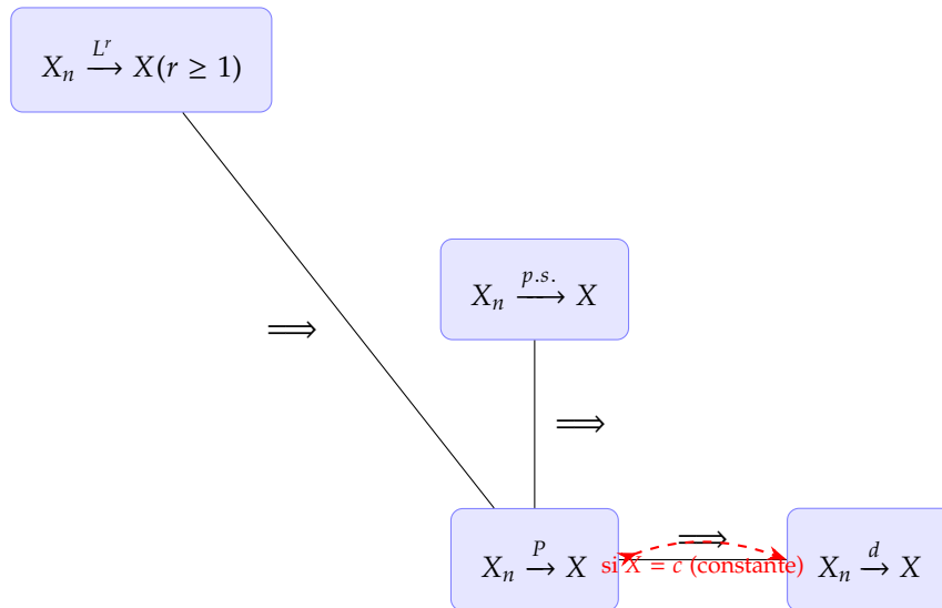
FIGURE 5.1 – Relations entre les modes de convergence.
