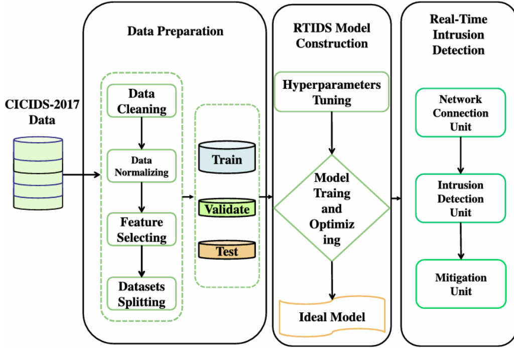
Figure 3.3: RTIDS model architecture [49]
