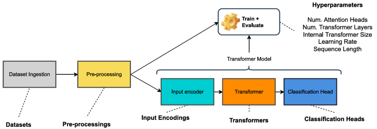
Figure 3.5: FlowTransformer framework architecture [51].
