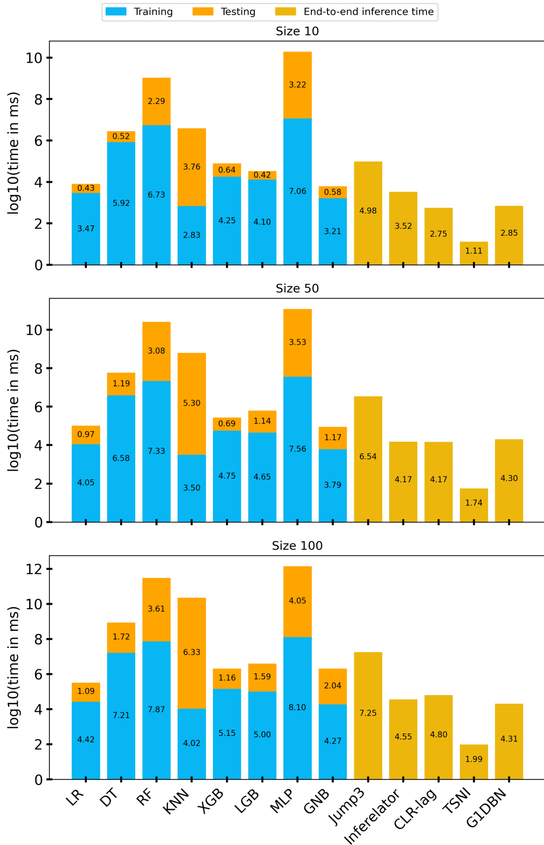
FIGURE 3.5: Comparison of running time across different GRN inference methods on the E. coli dataset for network sizes 10, 50, and 100. The y-axis shows the logarithm base 10 of the running time measured in milliseconds, while the x-axis represents the evaluated inference methods. Results highlight the trade off between higher initial training cost and faster inference for learning-based methods, particularly in scenarios involving repeated network inference.
