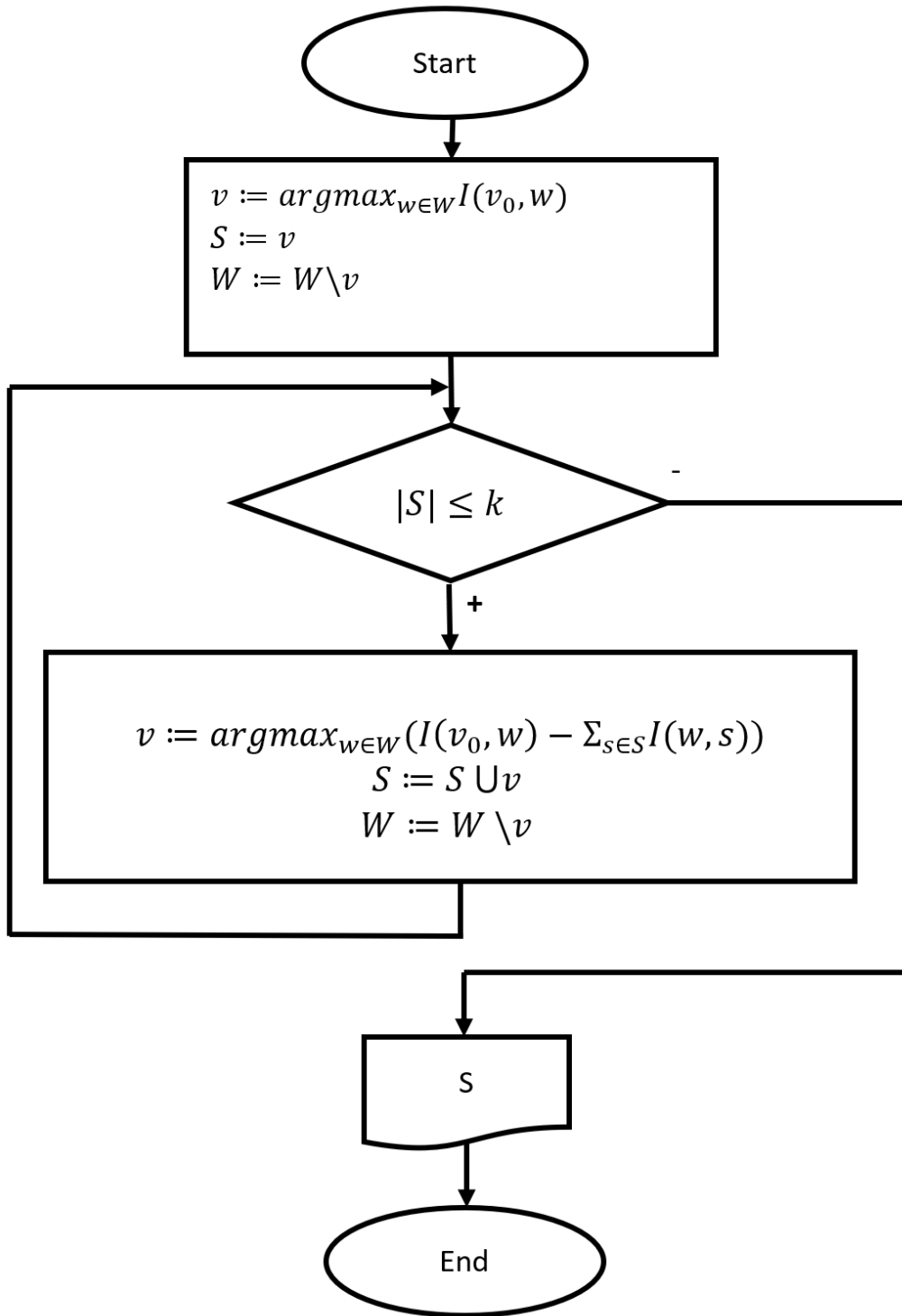
FIGURE 2.3: The subroutine MIFS(v_0, W, k) , where v_0 is the target variable, W = \{w_1, w_2, \dots, w_M\} is the set of variables, and k is the desired number of input variables.
