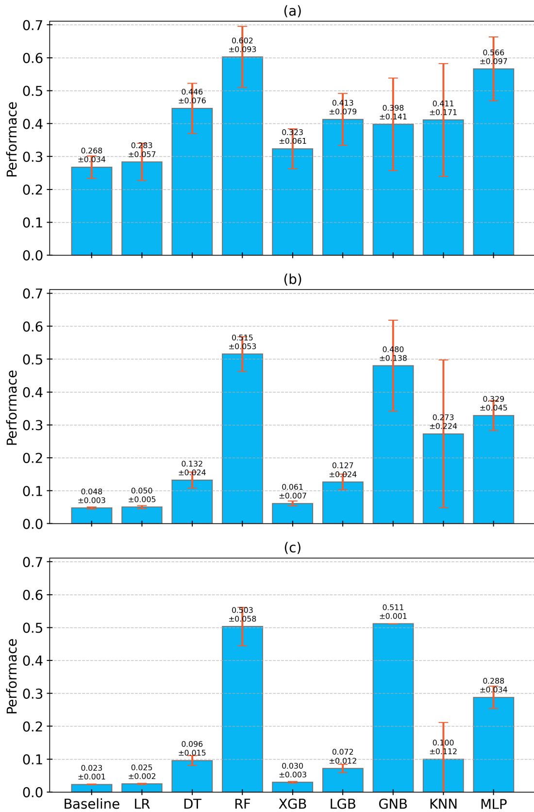
FIGURE 3.2: Figure shows the AUPR performance of different methods along the X-axis on the toy datasets. The Y-axis indicates the average AUPR values, with error bars representing the standard deviation. Subplots (a), (b), and (c) correspond to network sizes 10, 50, and 100, respectively, evaluated on 2,000, 400, and 400 test networks.
