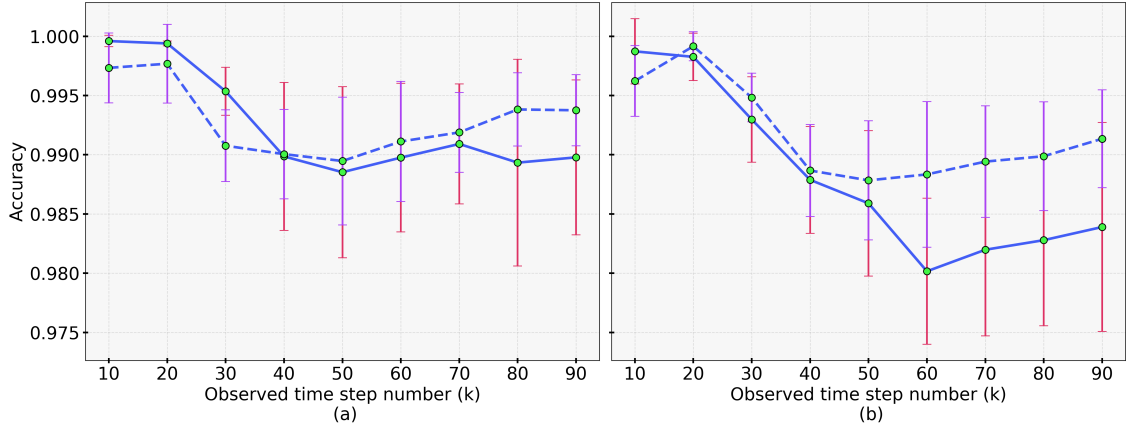
FIGURE 4.5: Comparison results of the dynamic accuracy on the Boolean discretization dataset. (a) Networks of |V| = 50 . (b) Networks of |V| = 100 . The Y-axis denotes the dynamic accuracy, and the X-axis indicates the number of observed time steps. The dashed and solid lines represent the results of the networks inferred from the original and the synthetic expression data, respectively.
