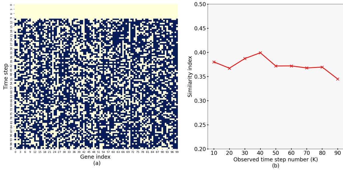
FIGURE 4.6: Similarity matrix between the synthesized gene expression data. (a) An example of a similarity matrix between a pair of synthesized gene expression data values when K equals 10. The white or black dot indicates that the corresponding gene values between two expression data values are identical or not, respectively. (b) Change in the mean similarity index against the time step number ( K ). For each K from 10 to 90, three pairs of synthesized gene expression data values were used to compute the mean similarity index. The Y-axis denotes the similarity index, defined as the rate of the number of identical dots over the total number of dots in the gene expression matrix. The X-axis corresponds to the number of observed time steps K .
