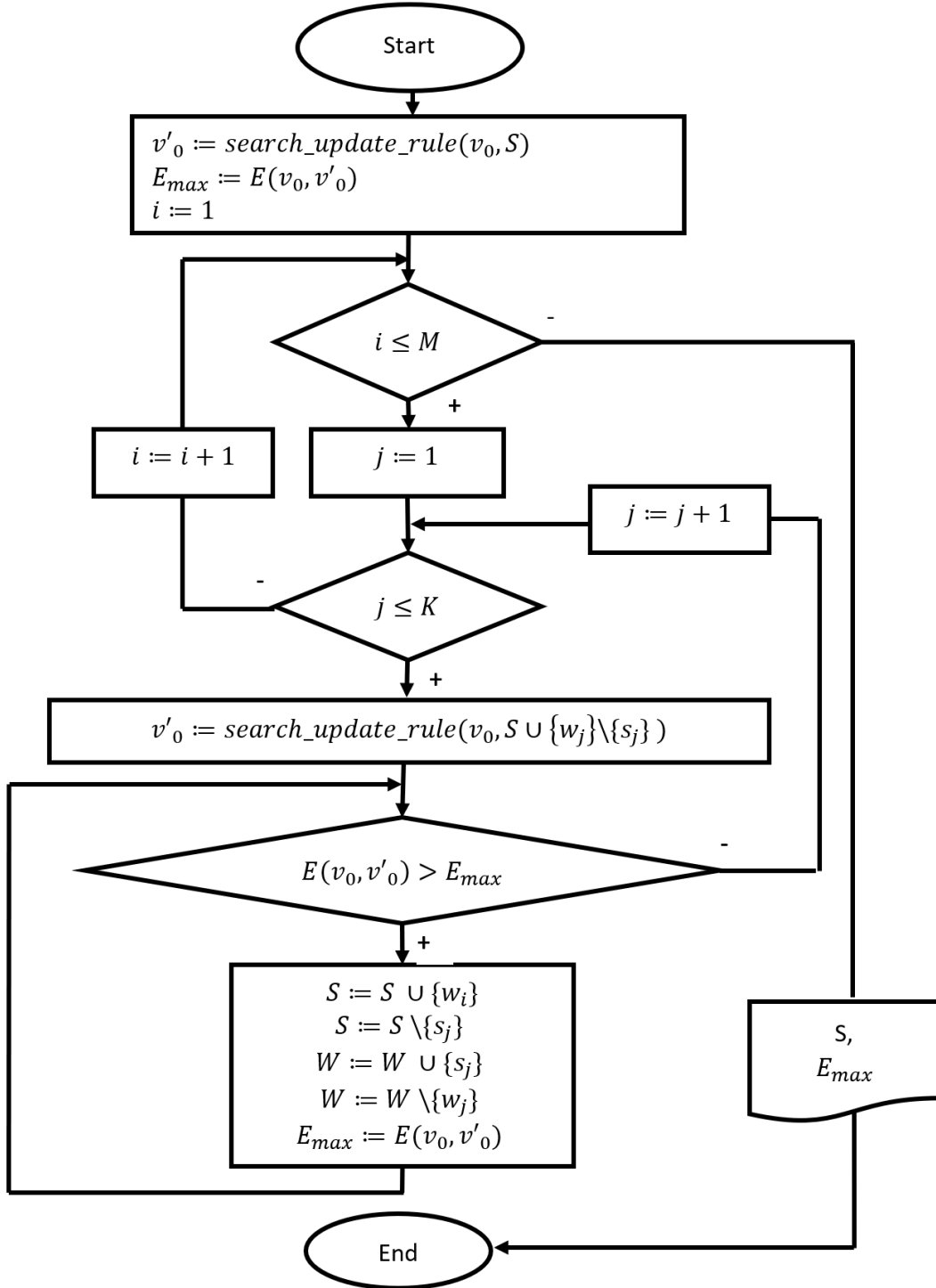
FIGURE 2.4: The subroutine SWAP(v_0, S, W) , where v_0 is the target variable; S = \{s_1, s_2, \dots, s_k\} is the set of selected variables such that I(v_0, s_i) \geq I(v_0, s_j) if i < j for all s_i, s_j \in S ; and W = \{w_1, w_2, \dots, w_M\} is the set of unselected variables such that I(v_0, w_i) \geq I(v_0, w_j) if i < j for all w_i, w_j \in W .
