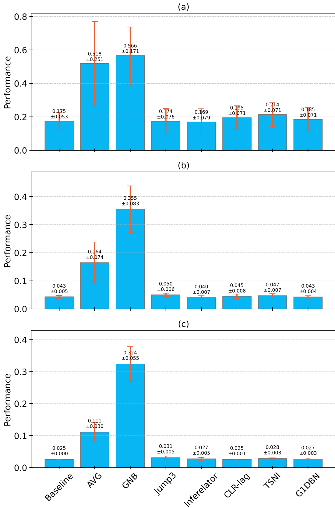
FIGURE 3.3: Figure shows the AUPR performance of different methods along the X-axis on the E.coli datasets. The Y-axis indicates the average AUPR values, with error bars representing the standard deviation. Subplots (a), (b), and (c) correspond to network sizes 10, 50, and 100, respectively, evaluated on 20, 8, and 8 test networks.
