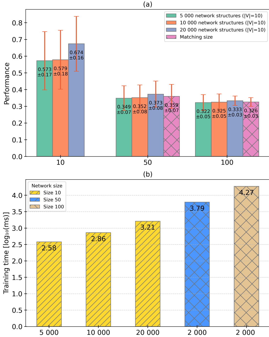
FIGURE 3.4: Performance and training-time analysis across varying training-set sizes and network scales. (a) Comparison of AUPR performance for three GNB models trained on datasets containing 5,000, 10,000, and 20,000 network structures (all with training network size of 10). Each model is evaluated on test networks of sizes 10, 50, and 100. Hatched bars denote the performance of models trained on matching network sizes (i.e., size-50 and size-100 training sets tested on size-50 and size-100 networks), included as baselines for comparison. The x-axis indicates the size of the testing network, and the y-axis reports AUPR. (b) Training-time comparison across datasets differing in both the number of network structures and the network size. The x-axis lists the training-set configurations (size-10 with 5 000, 10 000, and 20 000 structures, followed by size-50 and size-100 datasets, each has 2 000 network structures), and the y-axis reports the training time in \log_{10} -scaled milliseconds.
