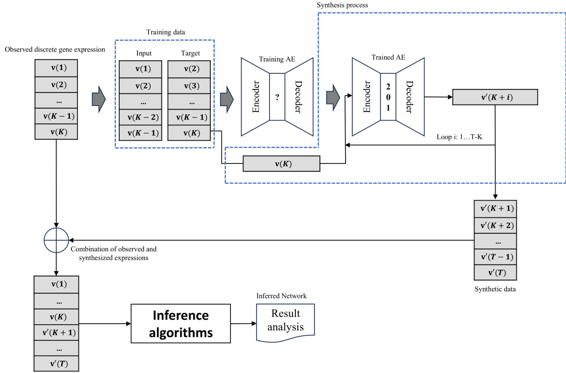
FIGURE 4.1: The framework of our method. The observed expression data create the input-target matrices, which represent a pair of consecutive expression vectors to train an autoencoder. The trained autoencoder autoregressively synthesizes expression data. The combined data of the observed and synthesized expressions are used as input for the inference algorithms.
