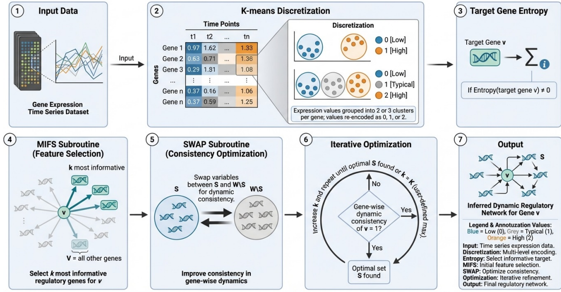
FIGURE 2.1: The overall framework of the MIDNI algorithm begins with a real-valued time-series gene expression dataset, which is transformed into a discretized expression dataset through the K-means discretization algorithm. The number of clusters K for each gene is adaptively determined using a validity index, ensuring that the discretization captures the inherent distribution of the gene's expression values. The discretized dataset is subsequently processed by the MIFS and SWAP subroutines, which identify the most informative regulatory genes for each target gene. The output of these subroutines is a collection of candidate regulatory sets for all genes in the network. Using these results, the gene regulatory network is reconstructed into a predictive network that can model and simulate the dynamic interactions among genes.
