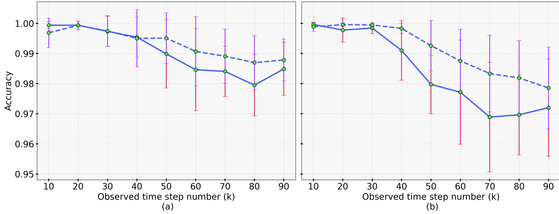
FIGURE 4.4: Comparison results of dynamic accuracy on the multi-level discretization dataset. (a) Networks of |V| = 50 . (b) Networks of |V| = 100 . The Y-axis denotes the dynamic accuracy, and the X-axis indicates the number of observed time steps. The dashed and solid lines represent the results of the networks inferred from the original and the synthetic expression data, respectively.
