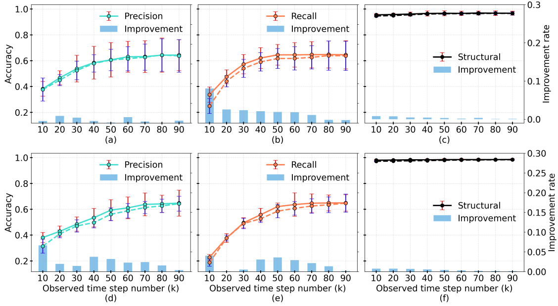
FIGURE 4.3: Results of precision, recall, and structural accuracy on the Boolean discretization dataset. (a–c) Results for the network with |V| = 50 . (d–f) Results for the network with |V| = 100 . The Y-axis denotes the performance metrics, and the X-axis indicates the number of observed time steps in the original gene expression data. For the synthesized dataset, gene expression data are generated for (100 - K) time steps. Solid and dashed lines represent the results based on the synthesized and the original dataset, respectively. Each point and error bar indicates the average value and the standard deviation, respectively, over 10 random networks. The bar charts show the performance improvement of the synthesized dataset over the original dataset.
