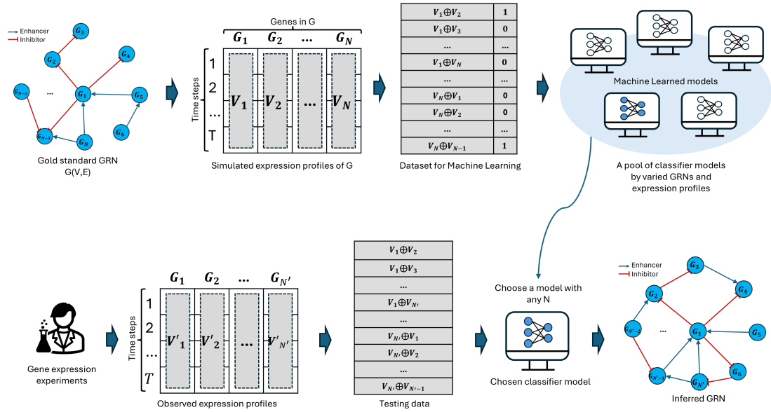
FIGURE 3.1: Overview of the proposed GRN inference framework. The key required input is the observed number of timesteps, which determines how simulated trajectories are aligned with the test instances. In contrast, network size is not a constraining factor, since the proposed representation enables models trained on networks of one size to generalize reliably to networks of different sizes. The framework produces pairwise interaction predictions for all gene pairs, which are then aggregated to reconstruct the inferred regulatory network.
