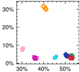
iImageNet-R200/10
