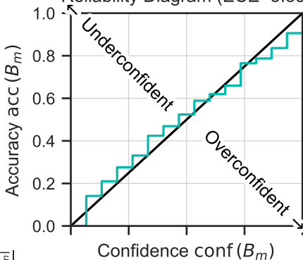
BALL iCIFAR100/10 Reliability Diagram (ECE=3.83)
