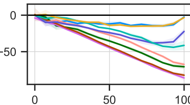
Bin B_m
