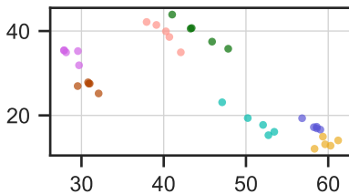
Avg. Acc. ↑
