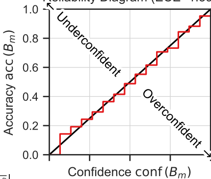
TBALL iCIFAR100/10 Reliability Diagram (ECE=1.39)
