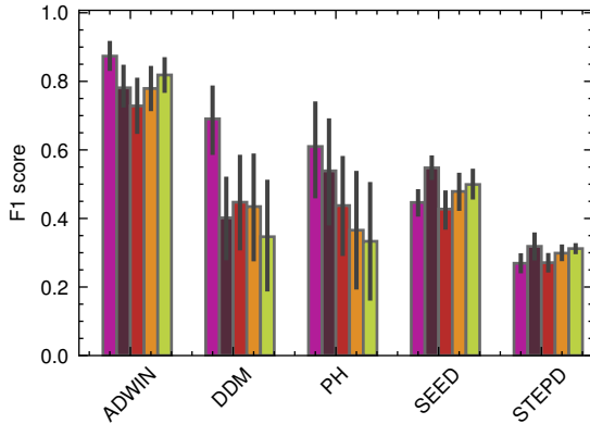
True Performance
