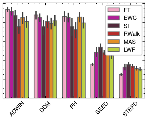
Estimated Performance
