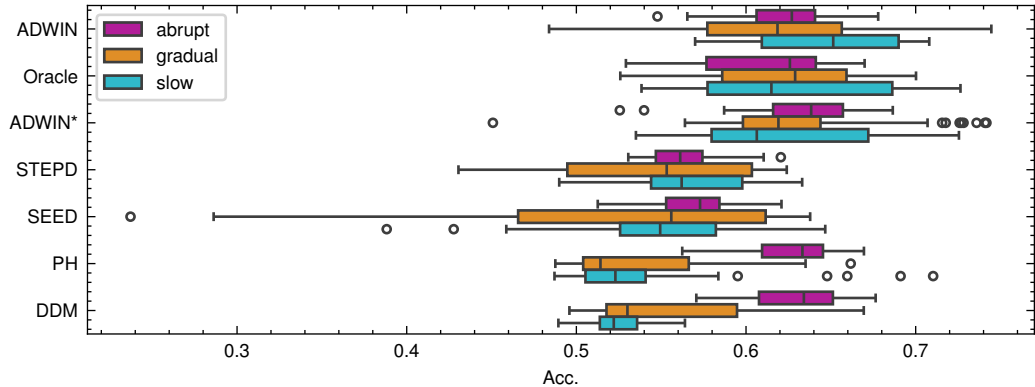
Acc. by Detector and Boundary
