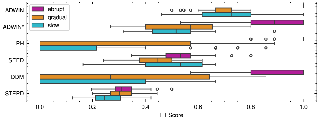
F1 Score by Detector and Boundary
