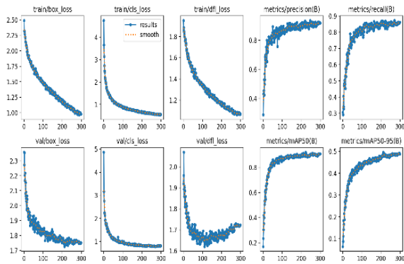
Fig. 2 Training and Validation Losses and Performance Metrics of YOLOv8n for Weapon Detection (Handgun, Knife, Shotgun) over 300 Epochs
