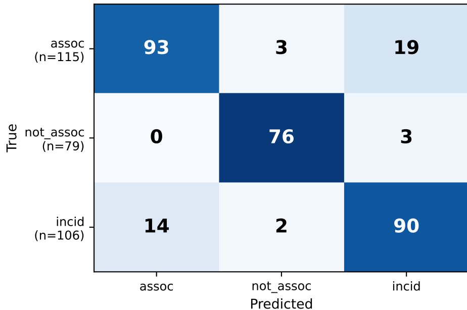
After label correction (v9, relabel4, 300 samples) Accuracy: 86.3%
