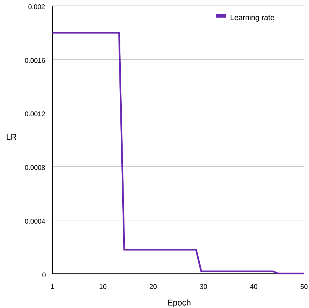
Learning-rate schedule
