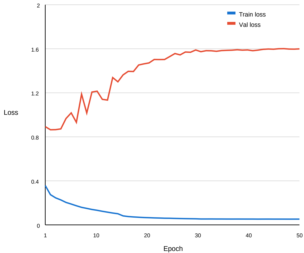
Faster R-CNN loss curves
