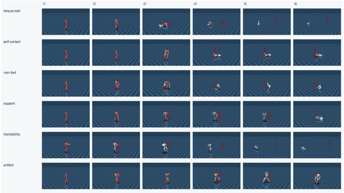
Figure 3: Representative generated-reference failures used in the slide deck. Rows correspond to torque/root-wrench demand, self-contact, non-foot floor contact, support proxy, controller trackability, and contact artifact. Each row shows six frames from the corresponding rollout video.
