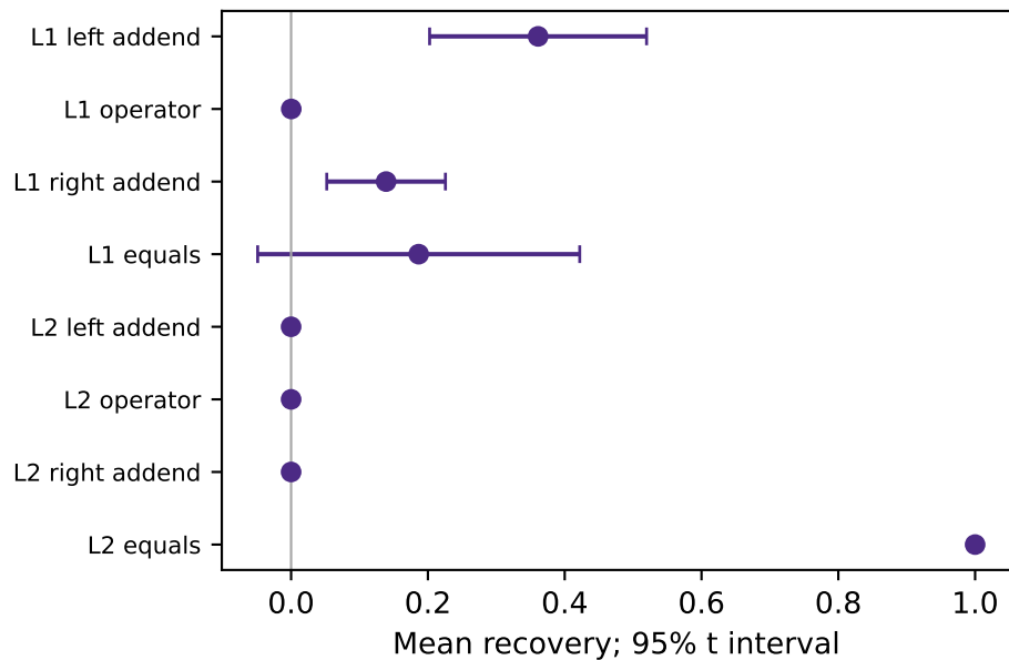
Seed-level uncertainty ( n = 4 )
