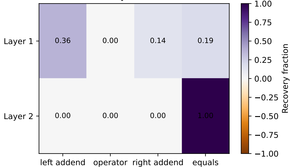
Mean recovery across four seeds
