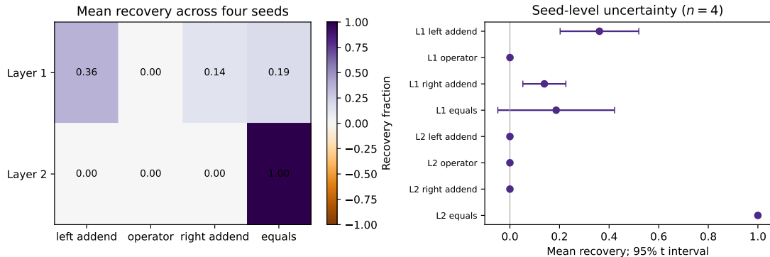
Figure 6: Four-seed causal residual-stream patching in the inspectable toy Transformer. The heat map gives mean clean-answer-logit recovery after inserting a clean residual state into a left-addend-corrupted run; points show the mean and two-sided 95% Student- t interval across four independent initializations. This figure is separate from the OpenAI artifact audit.
