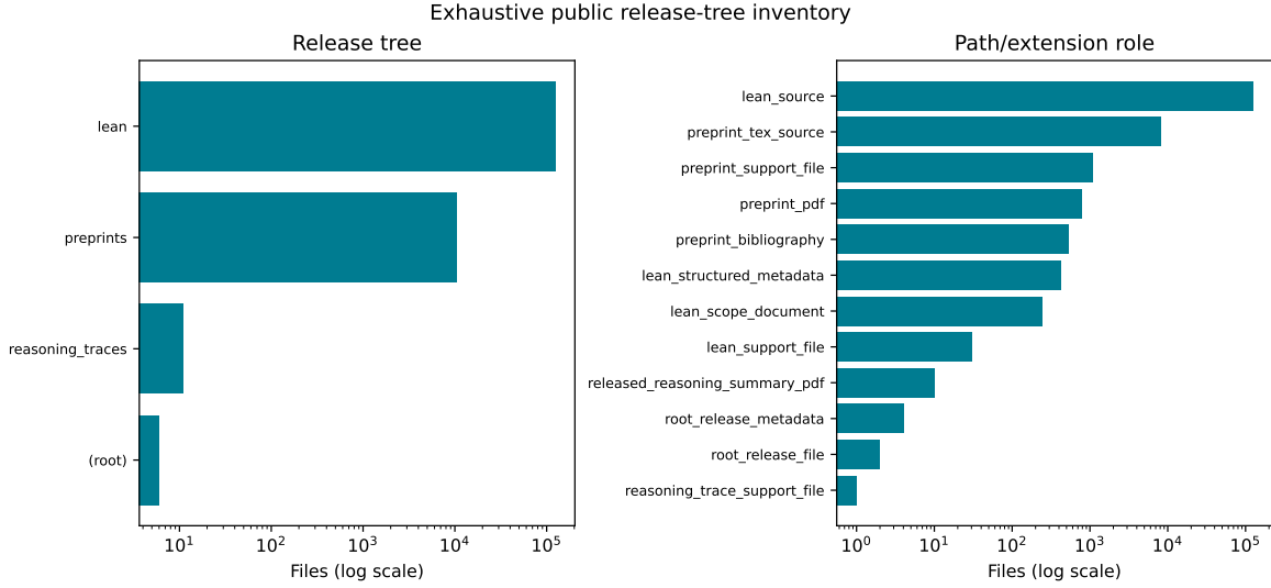
Figure 2: Complete path/extension-based inventory of the pinned release tree. The log scale makes the small root and reasoning-summary groups visible beside the large Lean and preprint collections. This is a structural census of all versioned blobs, not a quality or correctness assessment.
