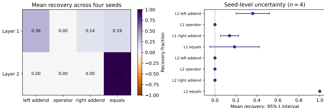
Figure 4: Four-seed causal residual-stream patching in the inspectable toy Transformer. The heatmap gives mean clean-answer-logit recovery after inserting a clean residual state into a left-addend-corrupted run; points show the mean and two-sided 95% Student- t interval across four independent initializations. This figure is separate from the OpenAI artifact audit.
