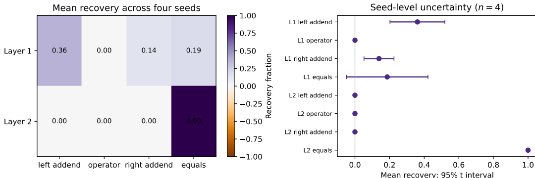
Figure 5: Four-seed causal residual-stream patching in the inspectable toy Transformer. The heat map gives mean clean-answer-logit recovery after inserting a clean residual state into a left-addend-corrupted run; points show the mean and two-sided 95% Student- t interval across four independent initializations. This figure is separate from the OpenAI artifact audit.
