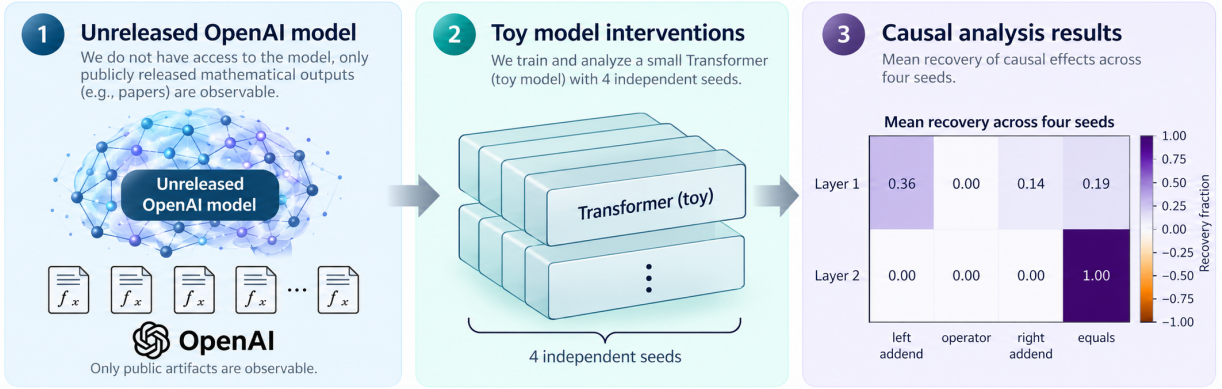
Figure 1: Overall conceptual workflow. The public OpenAI mathematics release supports an artifact audit but does not expose model internals. We therefore conduct causal residual-stream interventions only in separately trained, inspectable toy Transformers, then summarize recovery across four independent initialization seeds.
