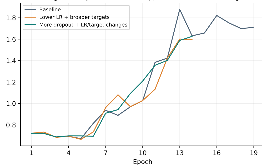
Higher dropout has not stopped evasion loss rising
