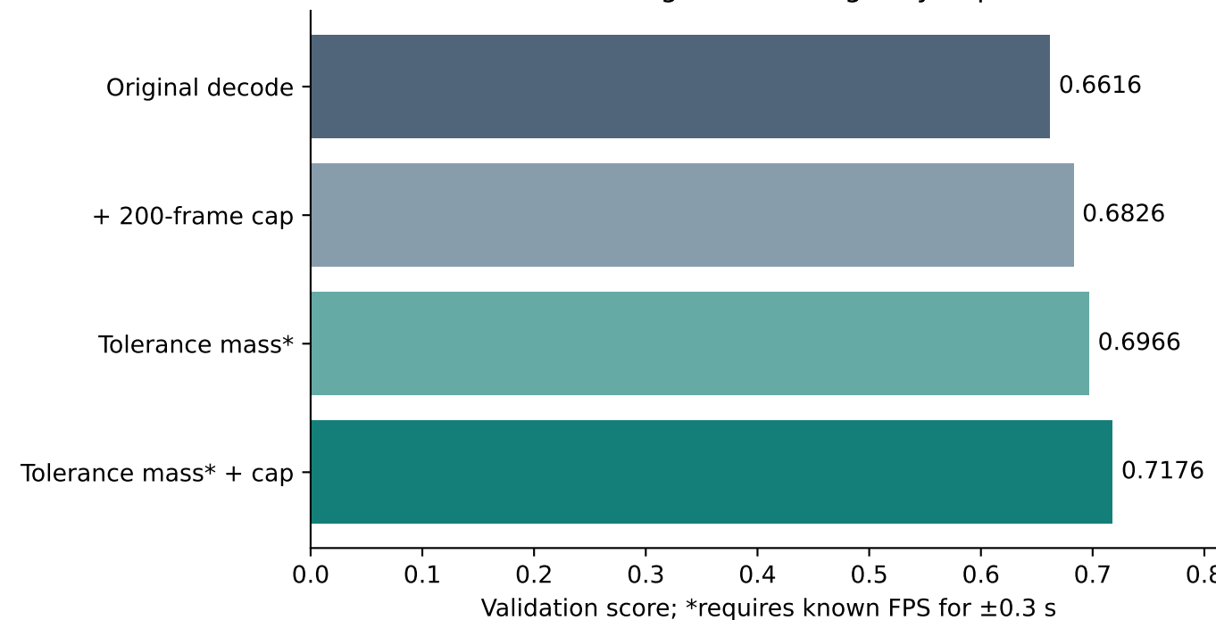
Same baseline logits: decoding-only experiments
