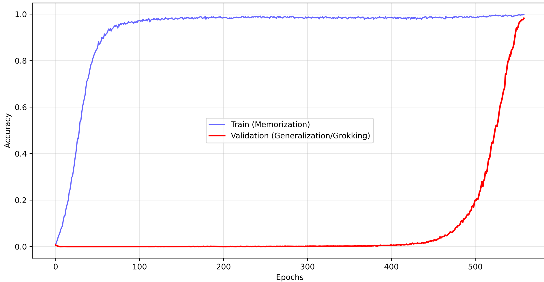
Looped LLM Grokking (Loops=4, P=97)
