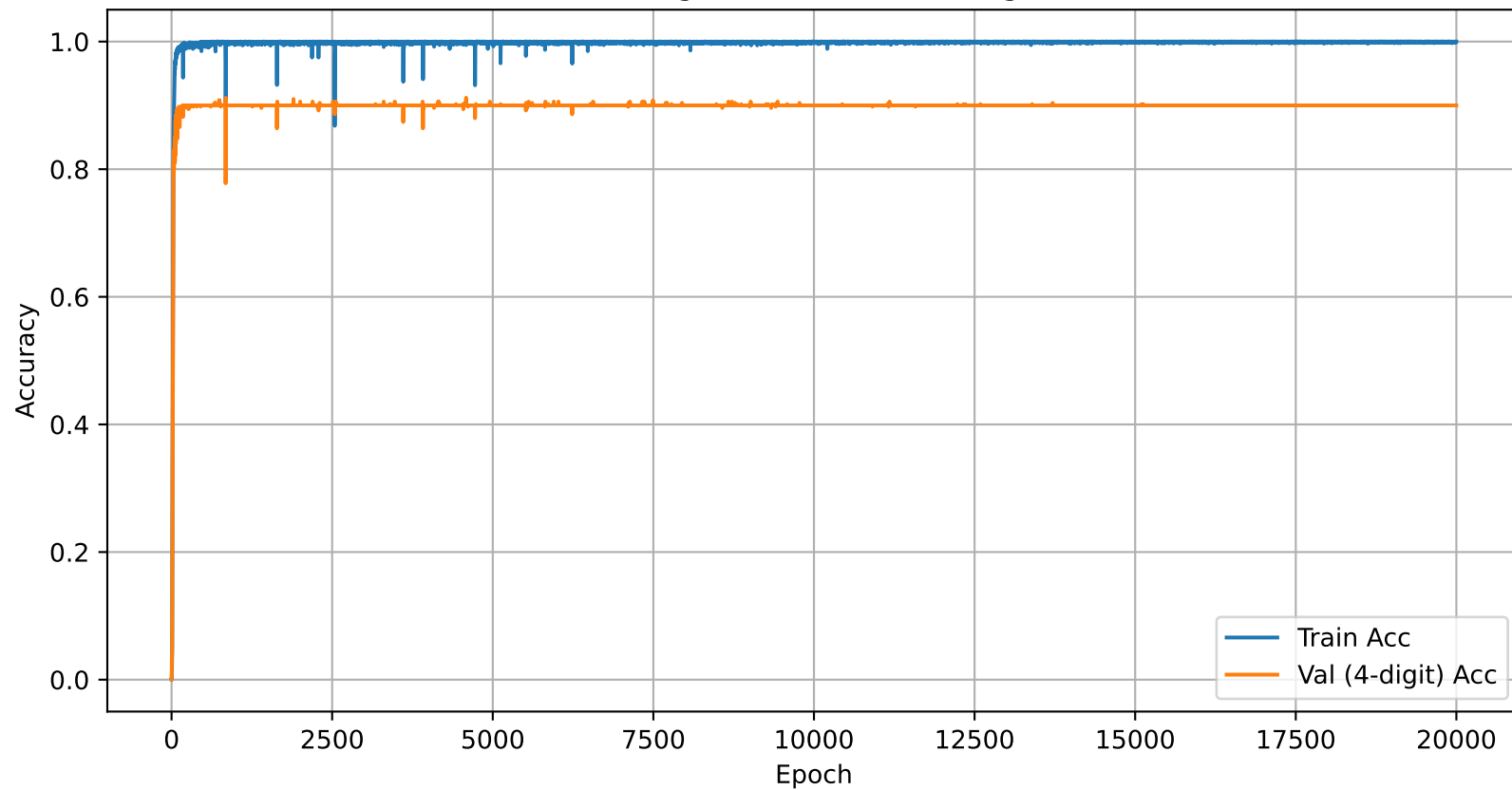
Grokking on Addition (4→8 digits)
