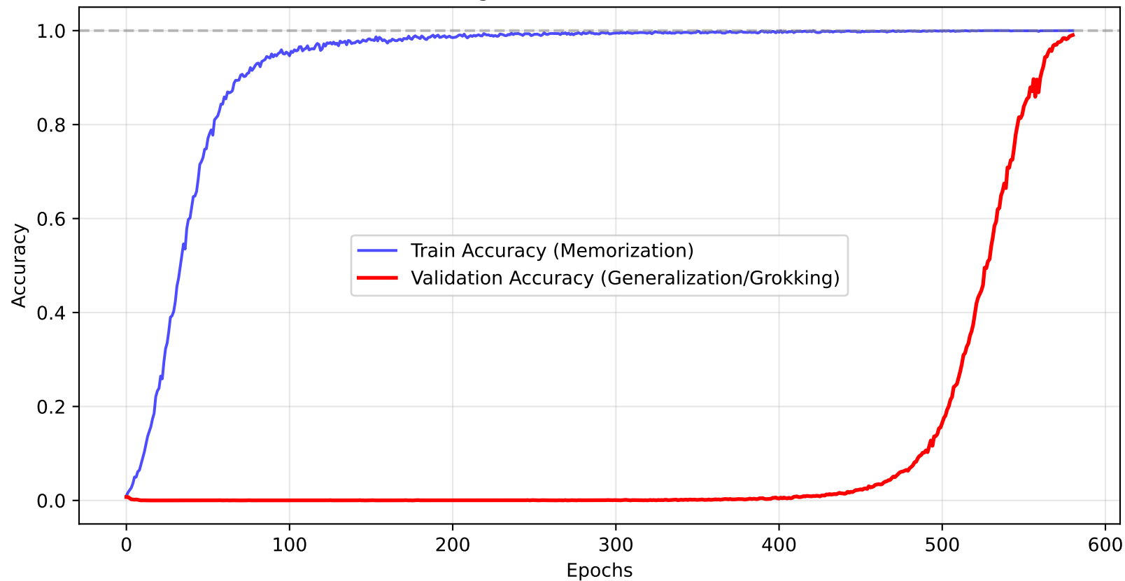
Grokking on Modular Addition (P=97)
