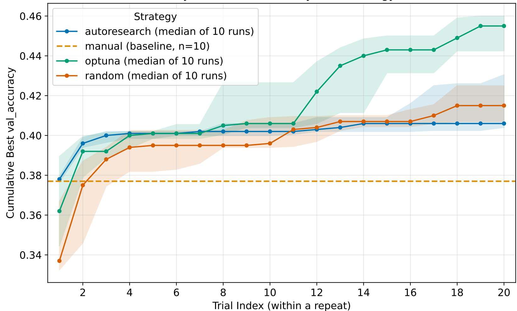
Anytime Performance by HPO Strategy
