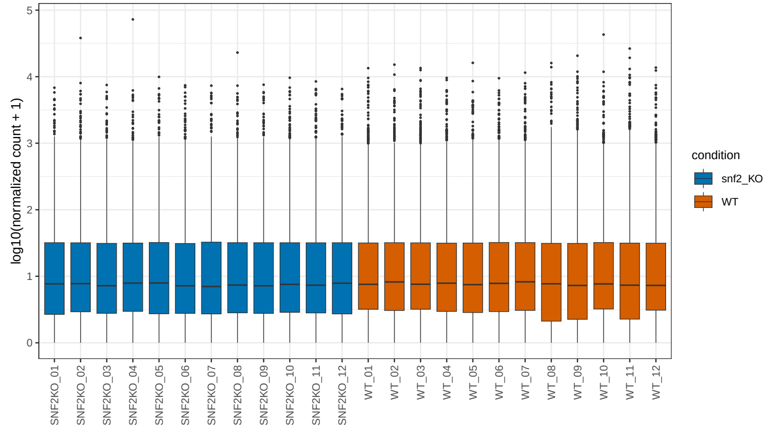
Normalized count distribution
