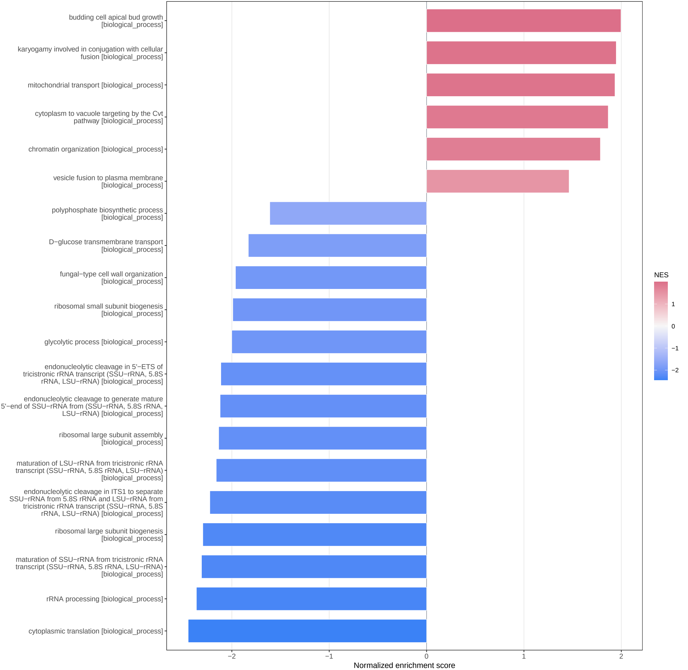
GSEA normalized enrichment scores Positive NES indicates enrichment near the top of the ranked gene list
