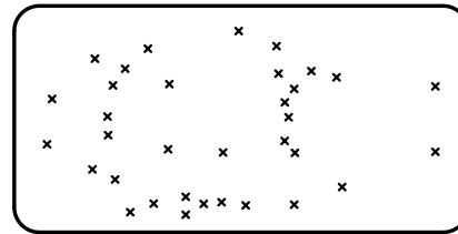
Drill Map: x 0.254mm / 0.0100" (34 holes)
