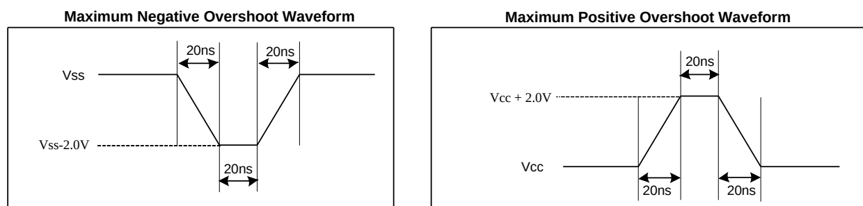
Figure 14. Overshoot Waveform
